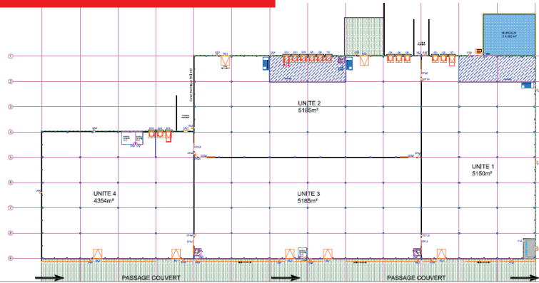
Construction phase 1 (section 1-4)
